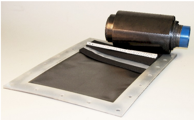
Picture 2: 2500 cm 2 redox flow cell and bipolar plate manufactured using roll-to-roll technique.
