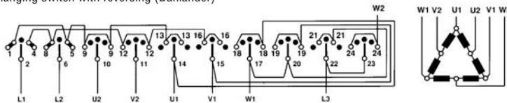
20 - Pole-changing switch with reversing (Dahlander)
