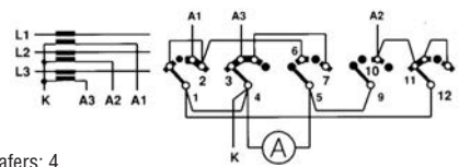
98 - L1-L2-L3 current changeover / double throw switch
