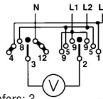
66 - Phase-phase phase-neutral voltmeter changeover / double throw
