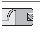
WN0 PTFE-Compound ≤ 5 bar, ≤ 25 m/s, -20 °C / +250 °C
