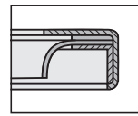
WP0 PTFE-Compound ≤ 7 bar, ≤ 25 m/s, -20 °C / +250 °C
