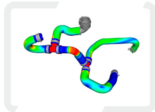
Piping of cooling hoses with clips and visualization of stresses
