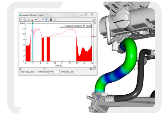
Analysis of stresses on a cooling hose
