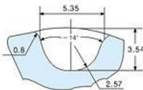
8M型齿形图: Tooth form diagram
