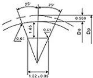
XL型齿形图: Tooth form diagram
