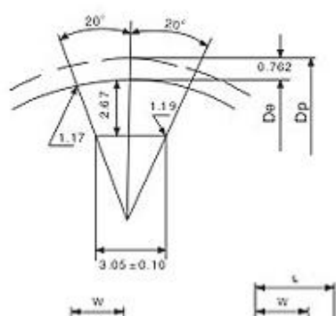
L型齿形图: Tooth form diagram
