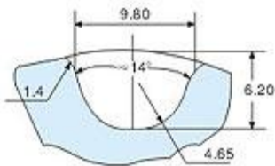
14M型齿形图: Tooth form diagram
