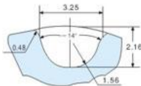
5M型齿形图: Tooth form diagram
