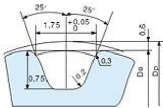
T2.5型齿形图: Tooth form diagram
