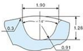
3M型齿形图: Tooth form diagram
