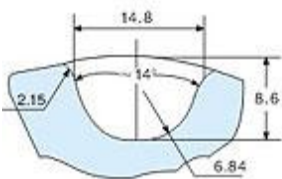
20M型齿形图: Tooth form diagram
