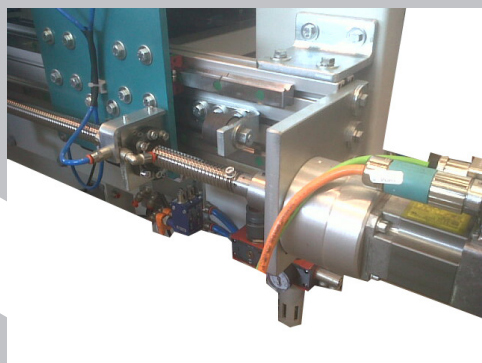
Squadra piano programmata Automatic fence with control by PLC
