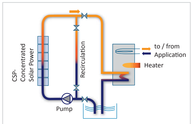
Schema einer Solarthermie-Hybridanlage Lay-out of Hybrid Solar Heat Process-Steam Plant
