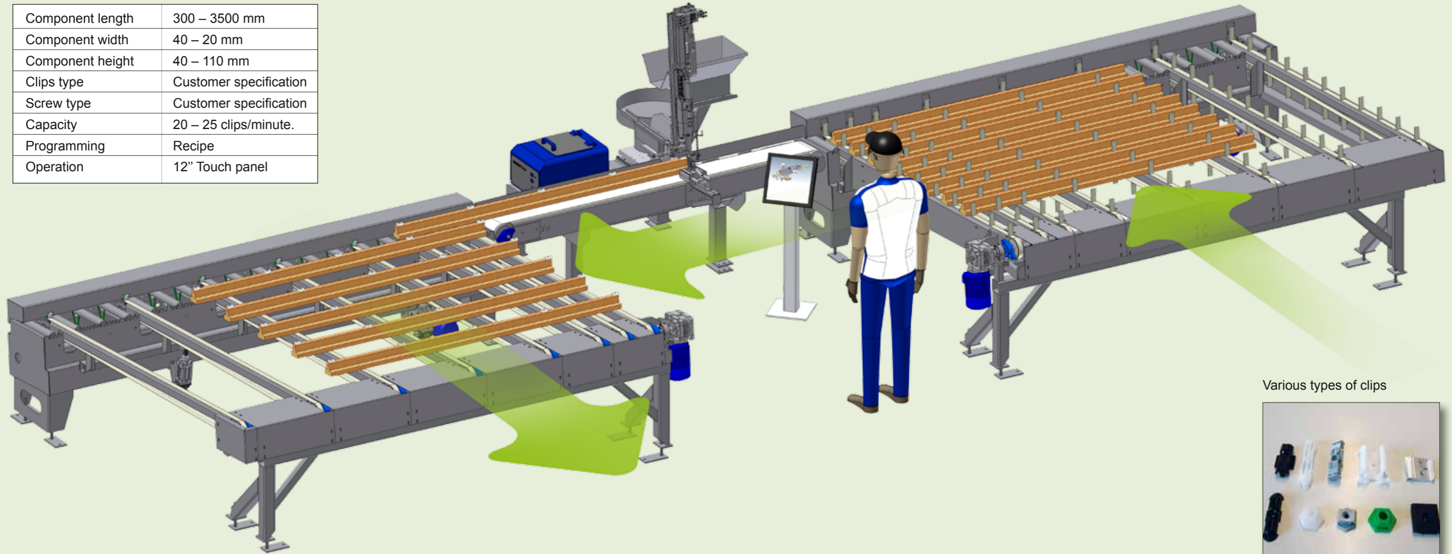
Clips mounting - side
