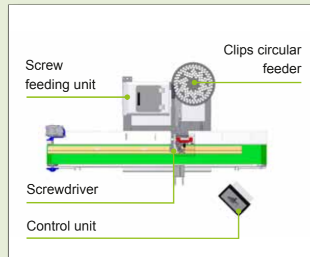
Clips mounting - top
