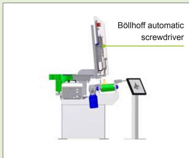
Clips mounting - side
