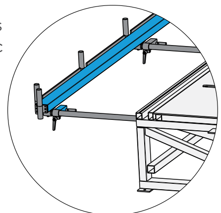
3D-view of the manual width adjustment with pneumatic squaring (BS2-MW3100P)
