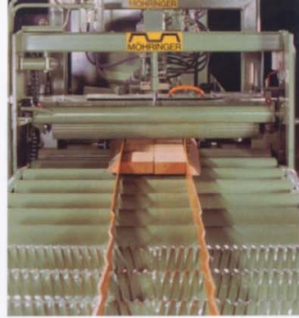
Outfeed separating conveyor
